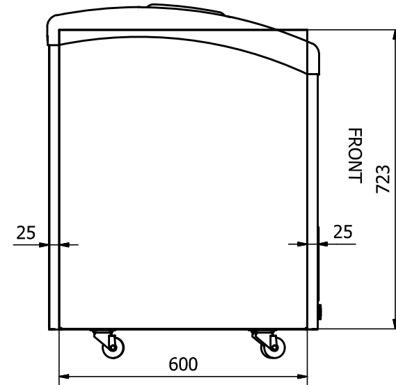
LEFT SIDE: Sticker 600 x 723 mm
